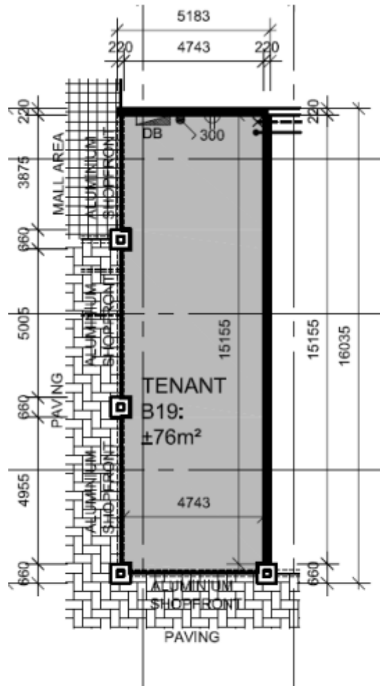
GROUND FLOOR PLAN Scale 1:200
